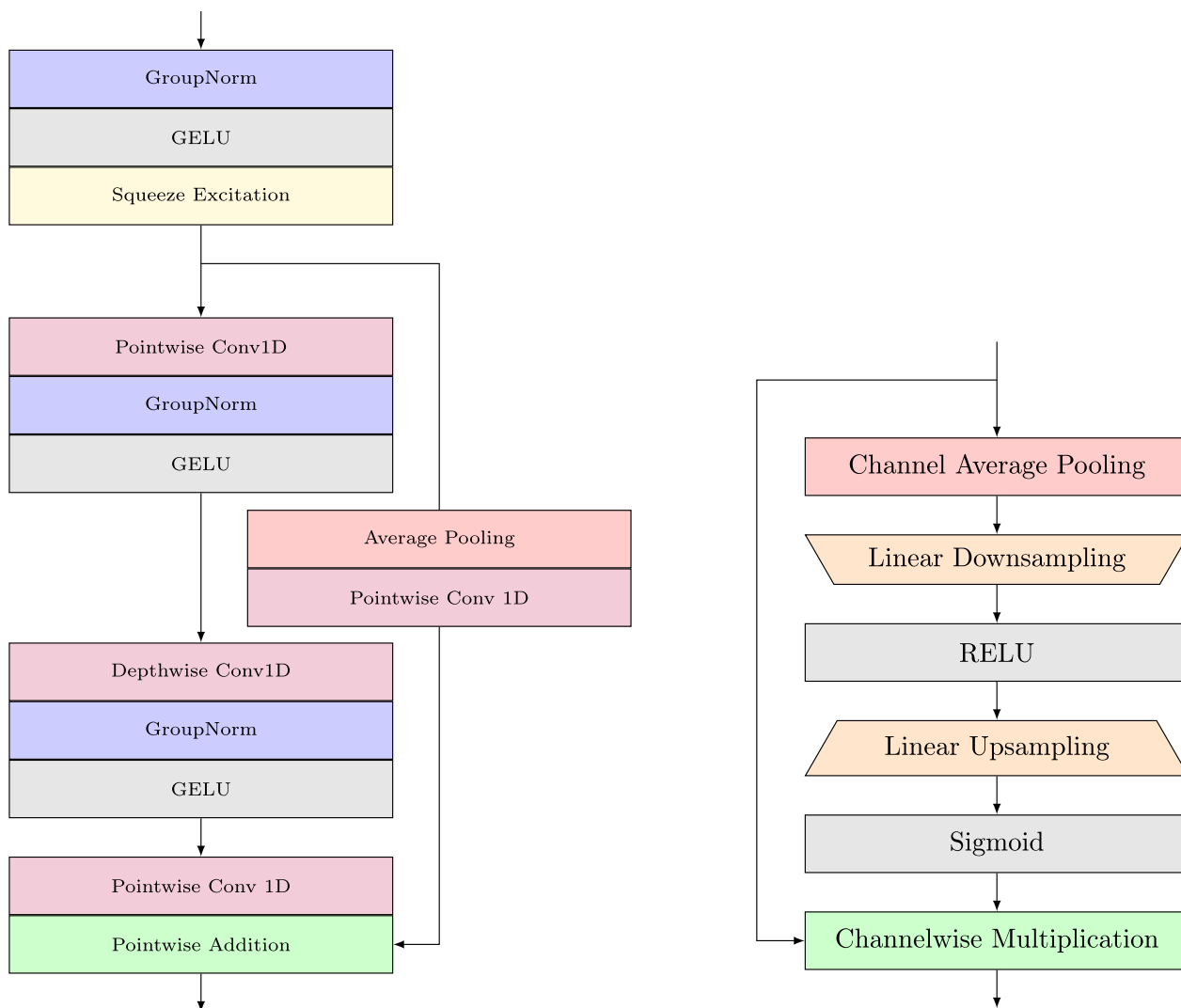
Fig. 6 Architecture of the residual block. Left The blocks use the pre-activation ResNet architecture with the addition of the GELU activation function and a squeeze-and-excitation layer. Right architecture of a squeeze-and-excitation block used to provide input dependant convolution filters
